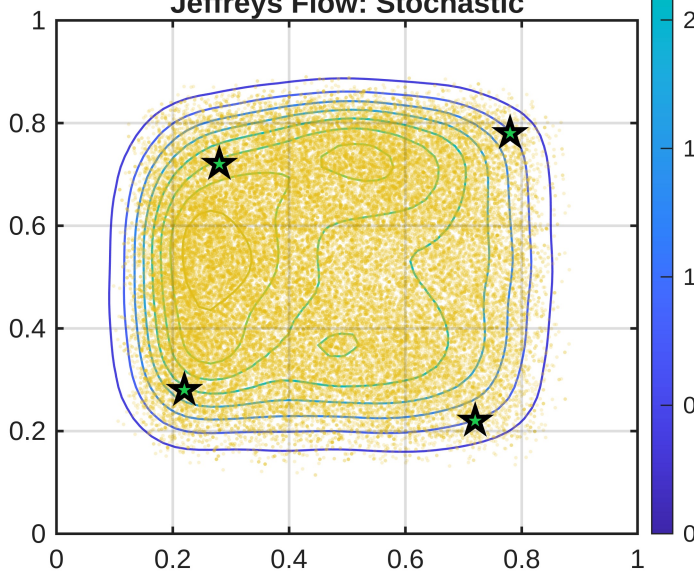
Jeffreys Flow: Stochastic
